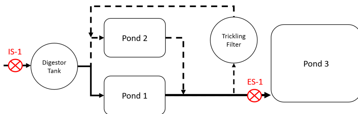
Figure 1. Process Flow Diagram with Sampling Locations
